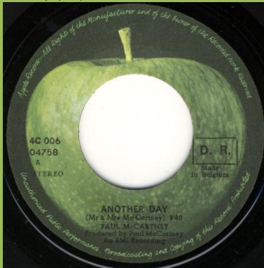
4C & 04758 aligned
